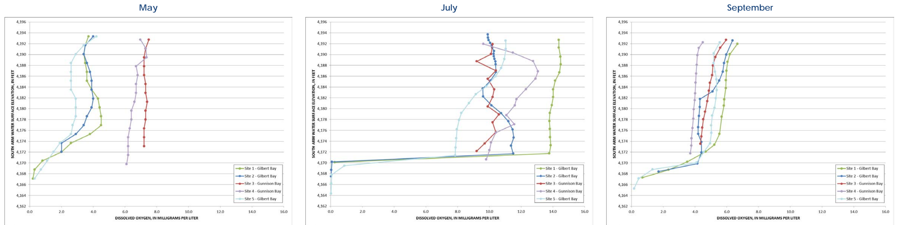
Figure 4. Dissolved Oxygen – 2014
