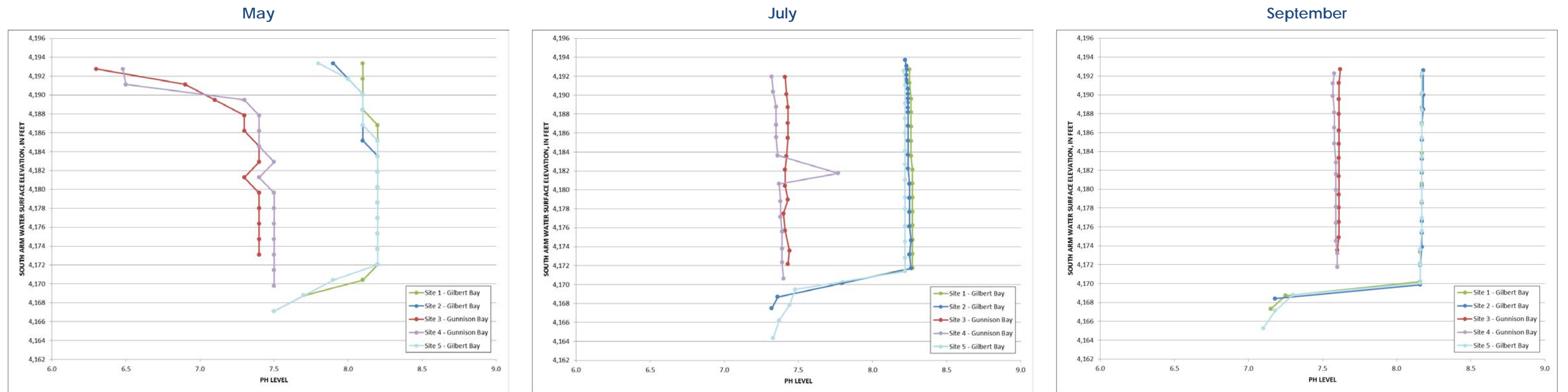
Figure 3. pH Profiles – 2014
