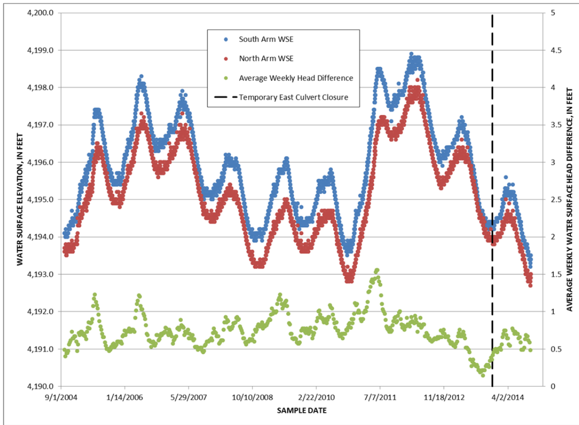
Figure 7. North and South Arm WSE and Head Difference
